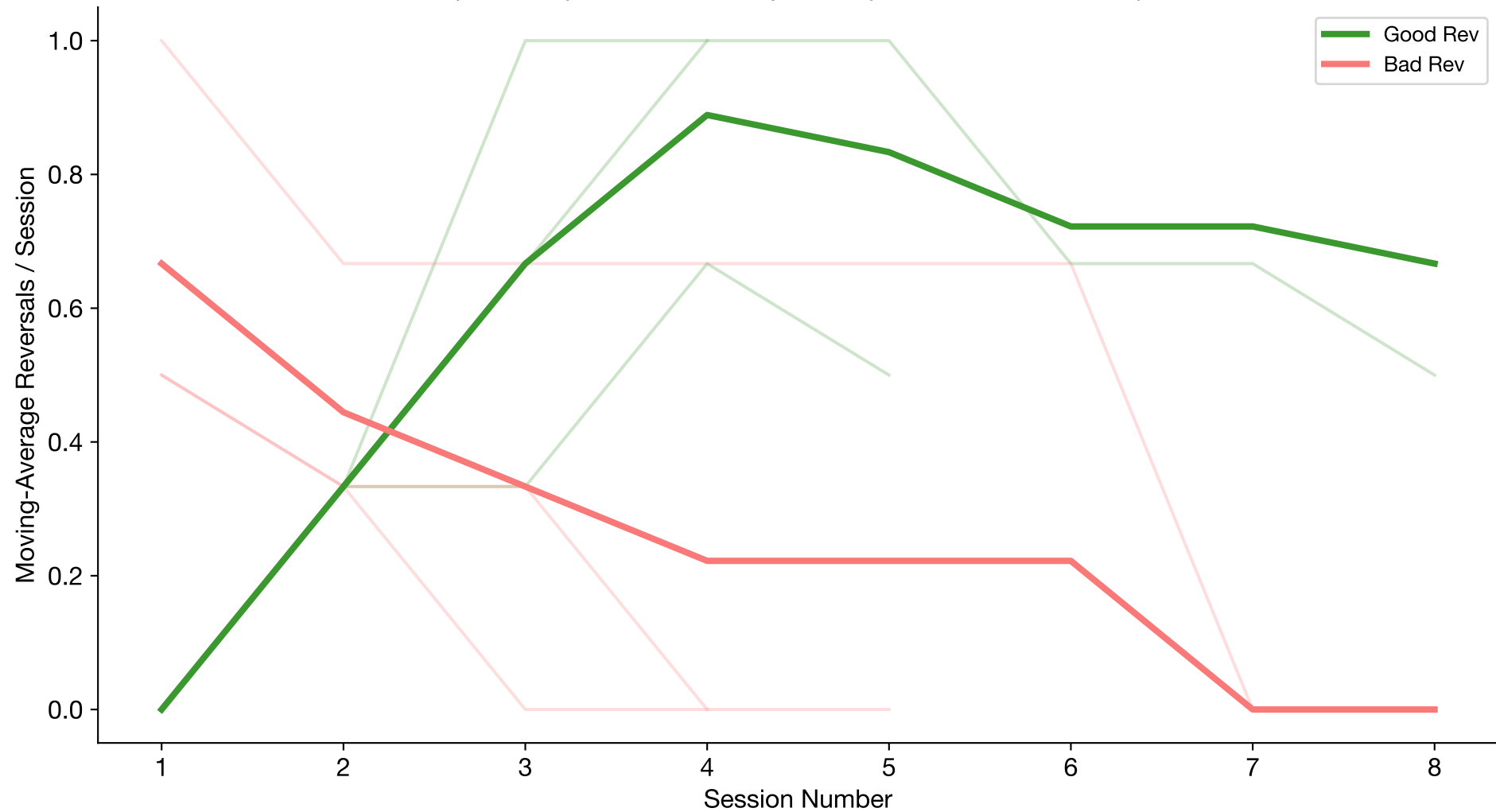
Moving-Average Good and Bad Reversals Over Time (n=3 subjects; sessions per subject=4–8; window=3)
